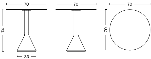
PALISSADE CONE TABLE Diameter 70 cm Height 74 cm Base diameter 33 cm Weight 37,9 kg
