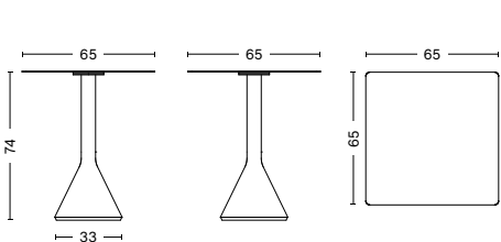
PALISSADE CONE TABLE Width 65 cm Depth 65 cm Height 74 cm Base diameter 33 cm Weight 37,9 kg
