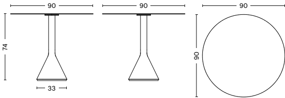
PALISSADE CONE TABLE Diameter 90 cm Height 74 cm Base diameter 33 cm Weight 44,6 kg
